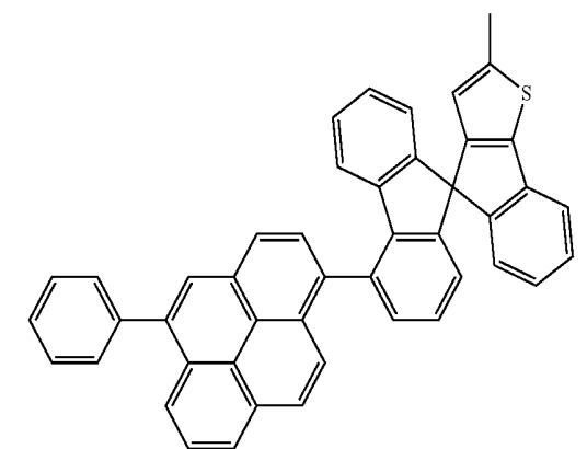
[Chemical Formula 48]
