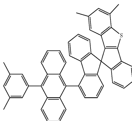
[Chemical Formula 16]
