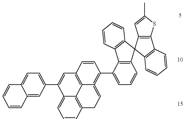
[Chemical Formula 50]
