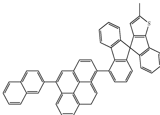
[Chemical Formula 50]
