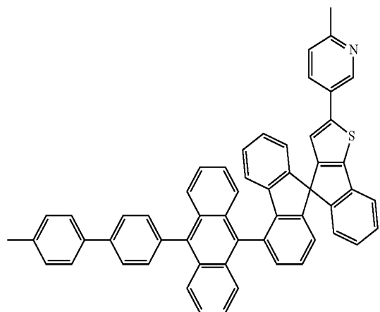
[Chemical Formula 46]
