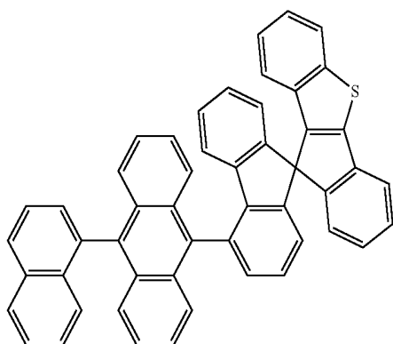
[Chemical Formula 30]
