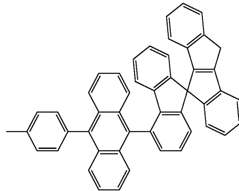
[Chemical Formula 63]
