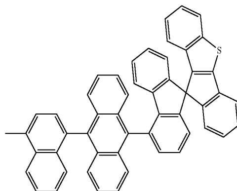
[Chemical Formula 30]
