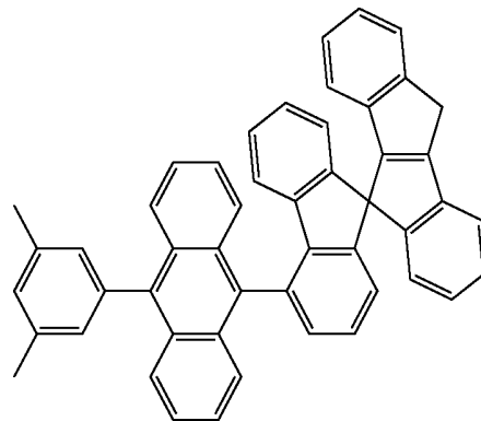
[Chemical Formula 64]
