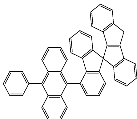
[Chemical Formula 63]
