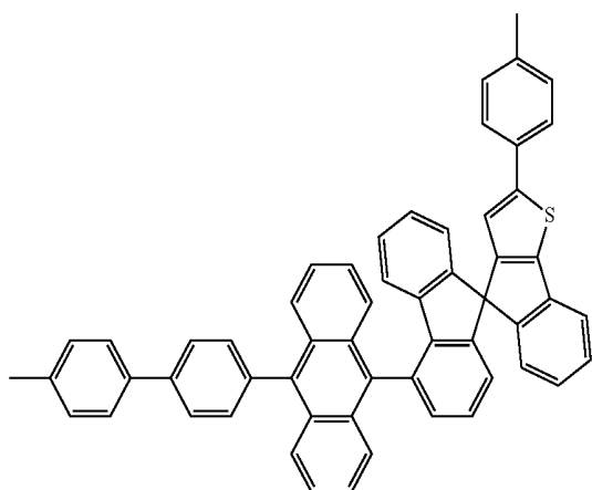
[Chemical Formula 42]
