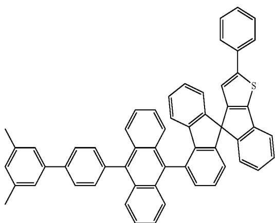
[Chemical Formula 43]
