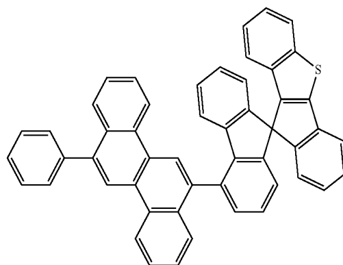
[Chemical Formula 52]
