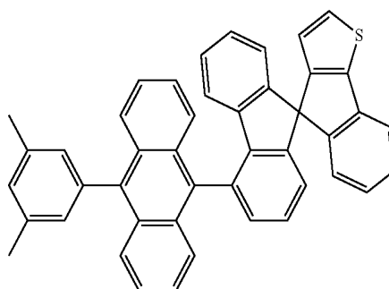
[Chemical Formula 5]
