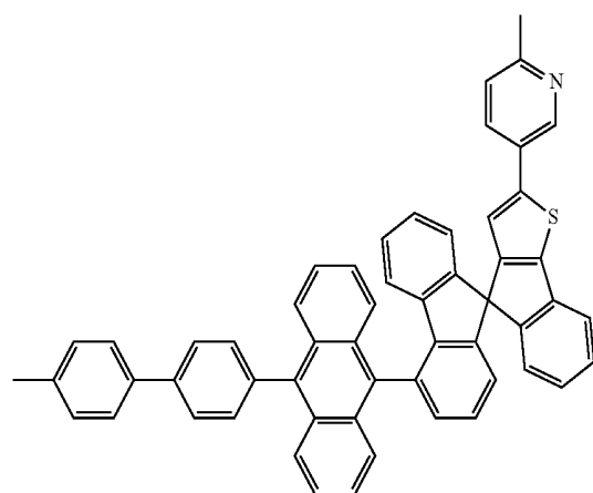
[Chemical Formula 46]
