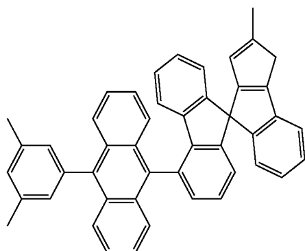
[Chemical Formula 62]
