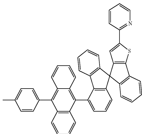
[Chemical Formula 10]
