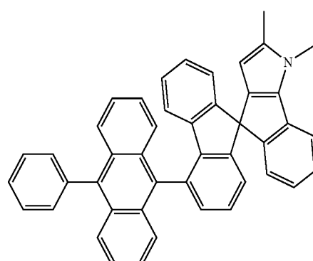
[Chemical Formula 65]
