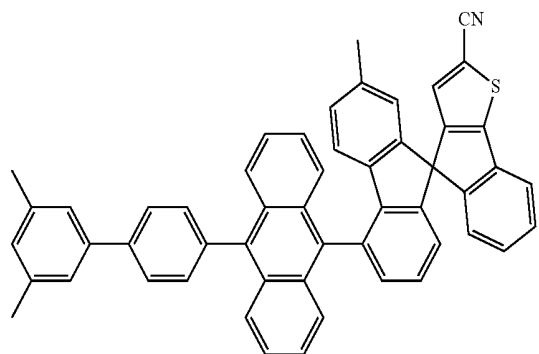
[Chemical Formula 47]
