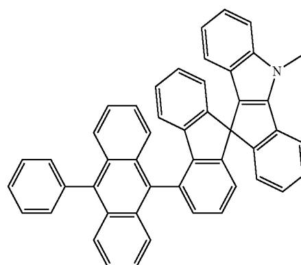
[Chemical Formula 68]
