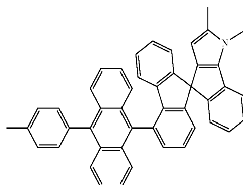
[Chemical Formula 67]
