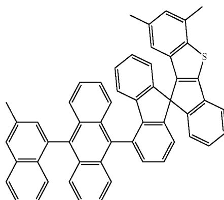
[Chemical Formula 34]
