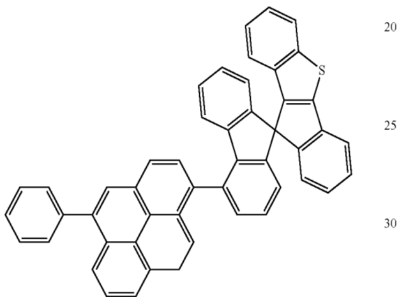
[Chemical Formula 51]
