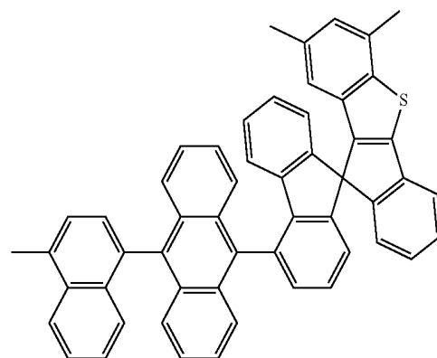
[Chemical Formula 34]
