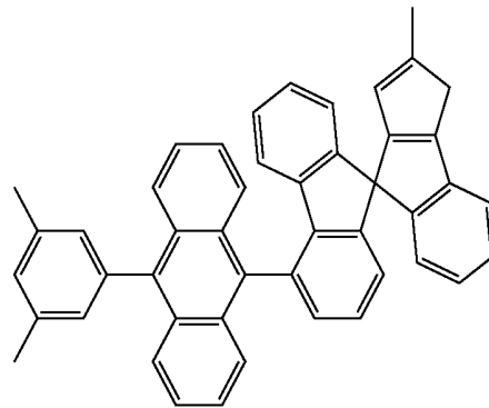
[Chemical Formula 62]
