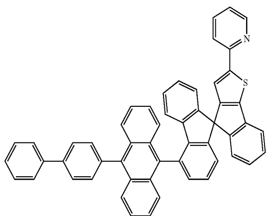
[Chemical Formula 44]
