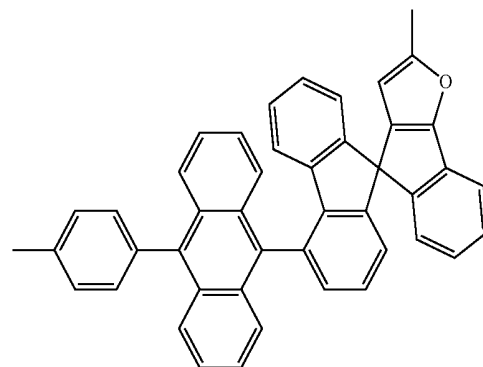
[Chemical Formula 54]
