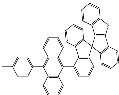
[Chemical Formula 12]
