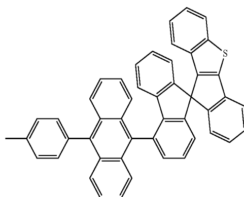
[Chemical Formula 12]
