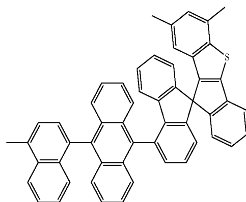
[Chemical Formula 34]
