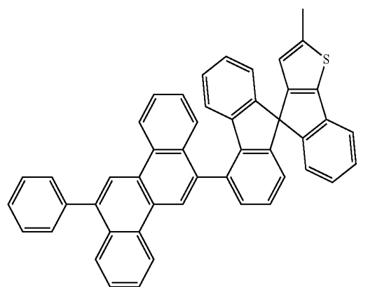
[Chemical Formula 48]
