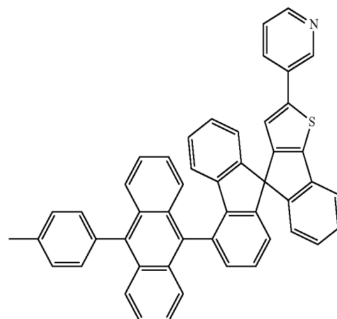
[Chemical Formula 8]
