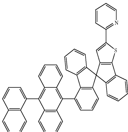
[Chemical Formula 28]
