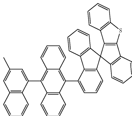
[Chemical Formula 32]
