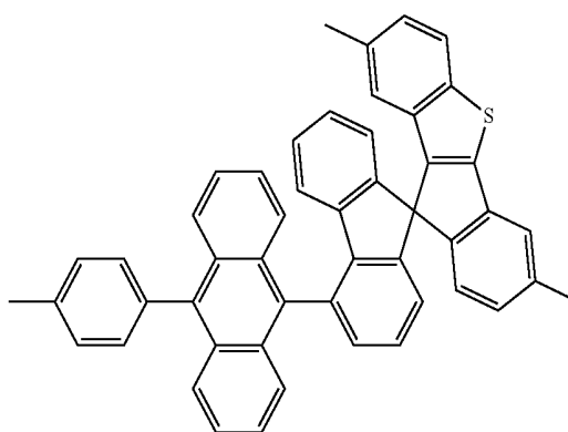
[Chemical Formula 16]
