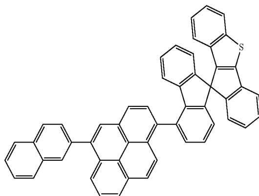
[Chemical Formula 52]
