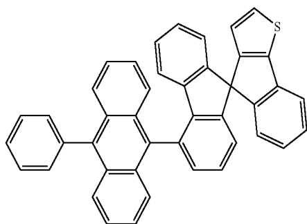
[Chemical Formula 3]
