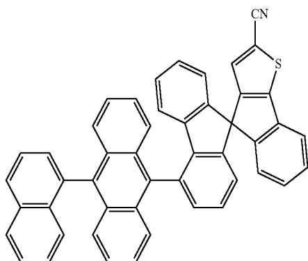
[Chemical Formula 29]
