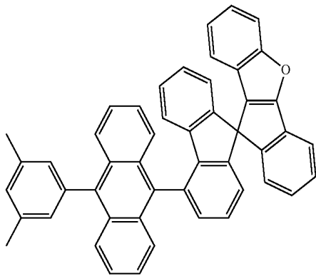
[Chemical Formula 59]
