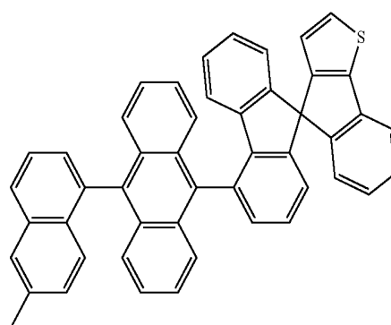
[Chemical Formula 23]
