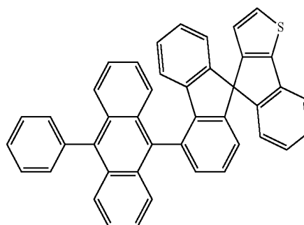
[Chemical Formula 2]
