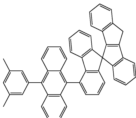
[Chemical Formula 64]
