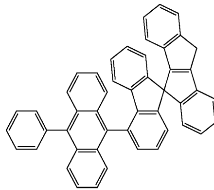
[Chemical Formula 63]
