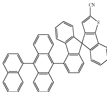
[Chemical Formula 29]
