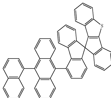
[Chemical Formula 30]
