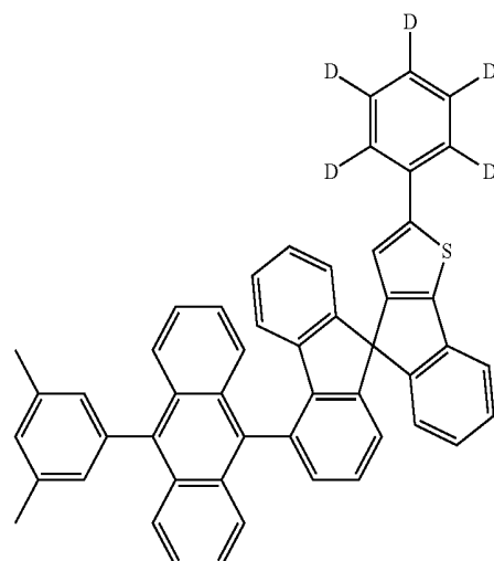
[Chemical Formula 7]
