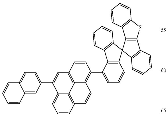
[Chemical Formula 52]
