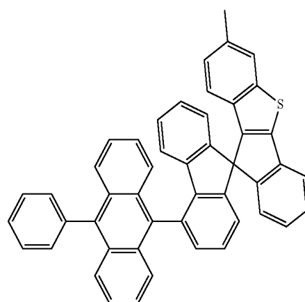
[Chemical Formula 15]
