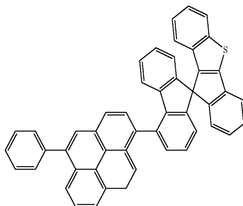
[Chemical Formula 51]
