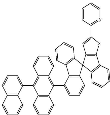
[Chemical Formula 28]
