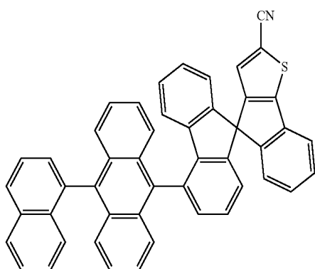
[Chemical Formula 29]
