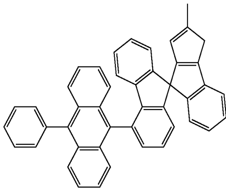
[Chemical Formula 59]
