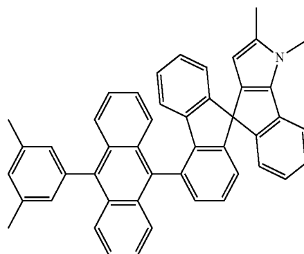
[Chemical Formula 68]
