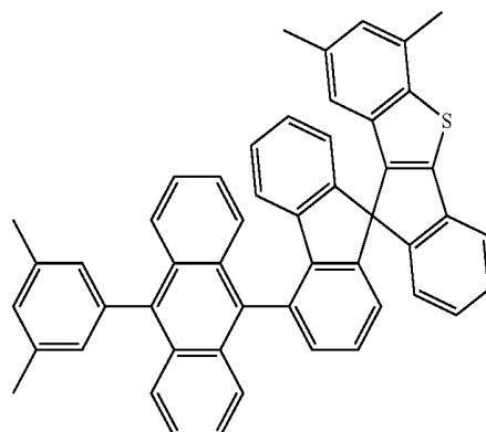
[Chemical Formula 16]
