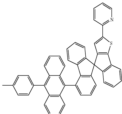
[Chemical Formula 10]
