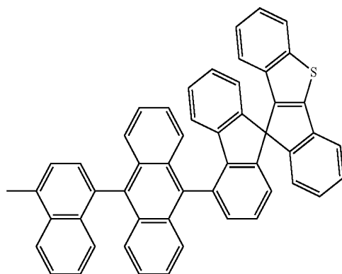
[Chemical Formula 30]
