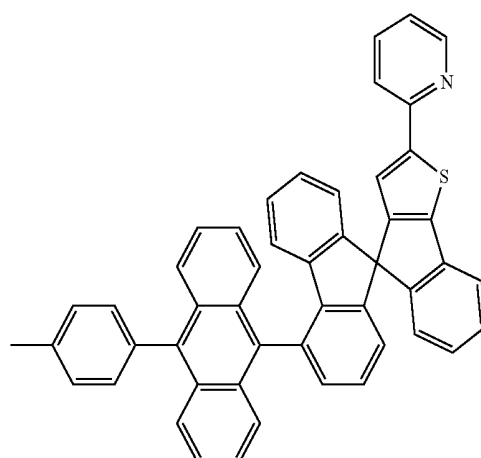
[Chemical Formula 10]
