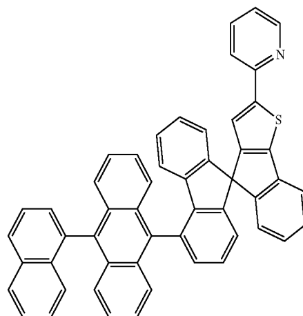
[Chemical Formula 28]
