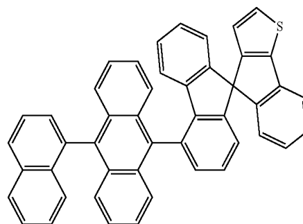
[Chemical Formula 20]
