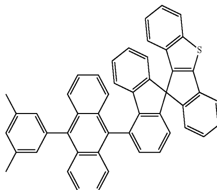
[Chemical Formula 14]
