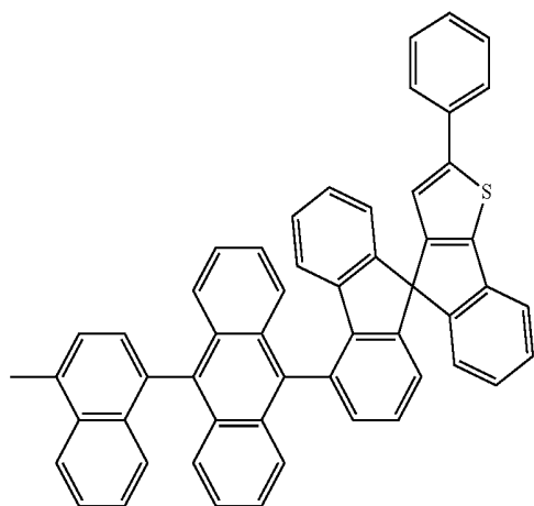
[Chemical Formula 25]
