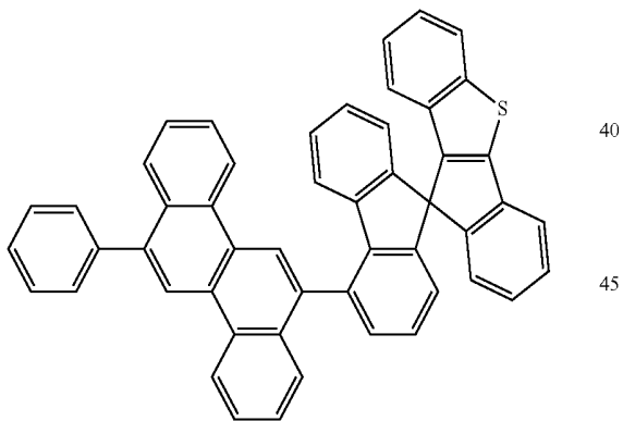
[Chemical Formula 52]
