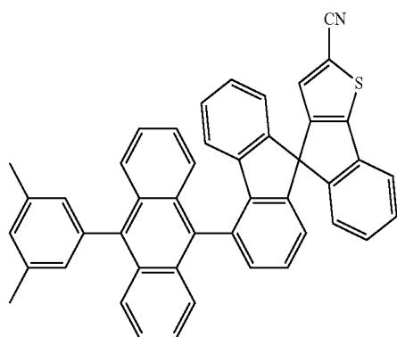
[Chemical Formula 11]
