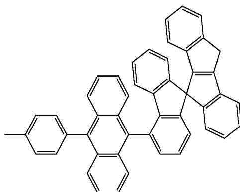
[Chemical Formula 63]
