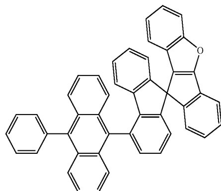
[Chemical Formula 56]
