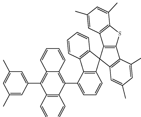
[Chemical Formula 17]
