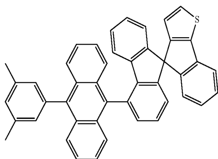
[Chemical Formula 4]
