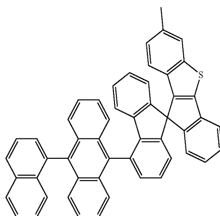
[Chemical Formula 33]
