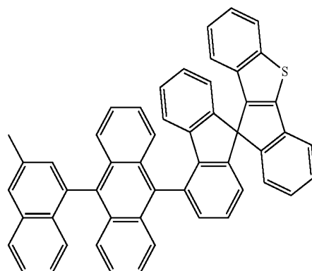
[Chemical Formula 32]
